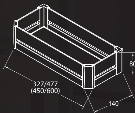
OUTER BASKET
