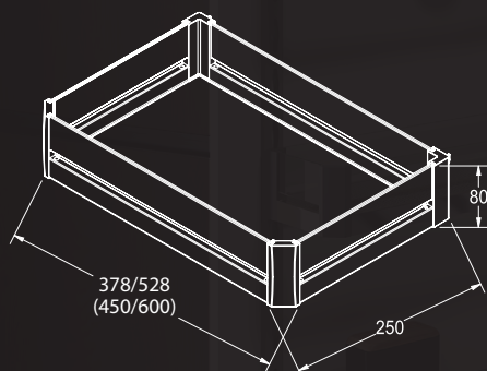
INNER BASKET
